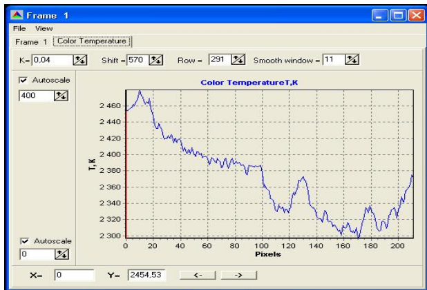
Fig. 4: Spatial profile of recalculated colour temperature at the irradiation spot.
