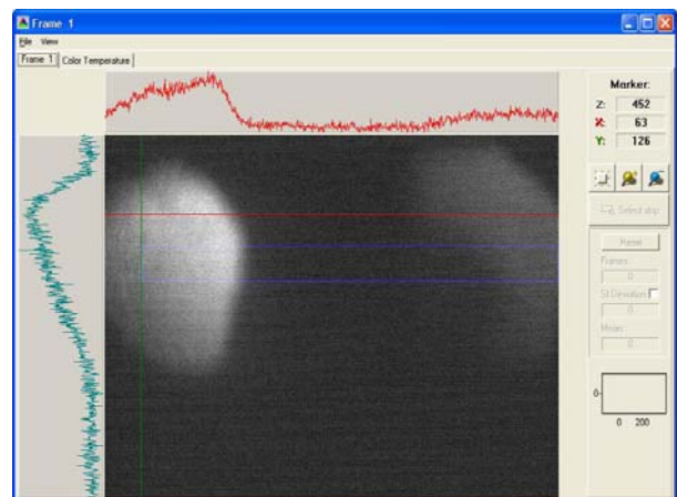
Fig.3: Spatial distribution of thermal radiation intensity at two wavelengths (left image is recorded at \lambda_2 = 0.7 \mu\text{m} and right
