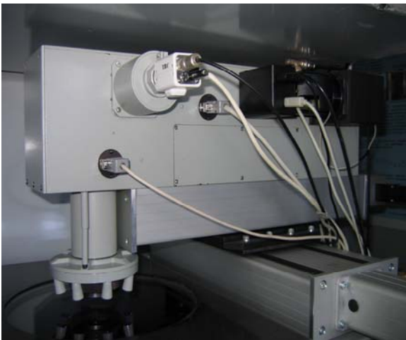
Fig.1: Opto-mechanical unit for process monitoring and on-line control of the SLS machine.
